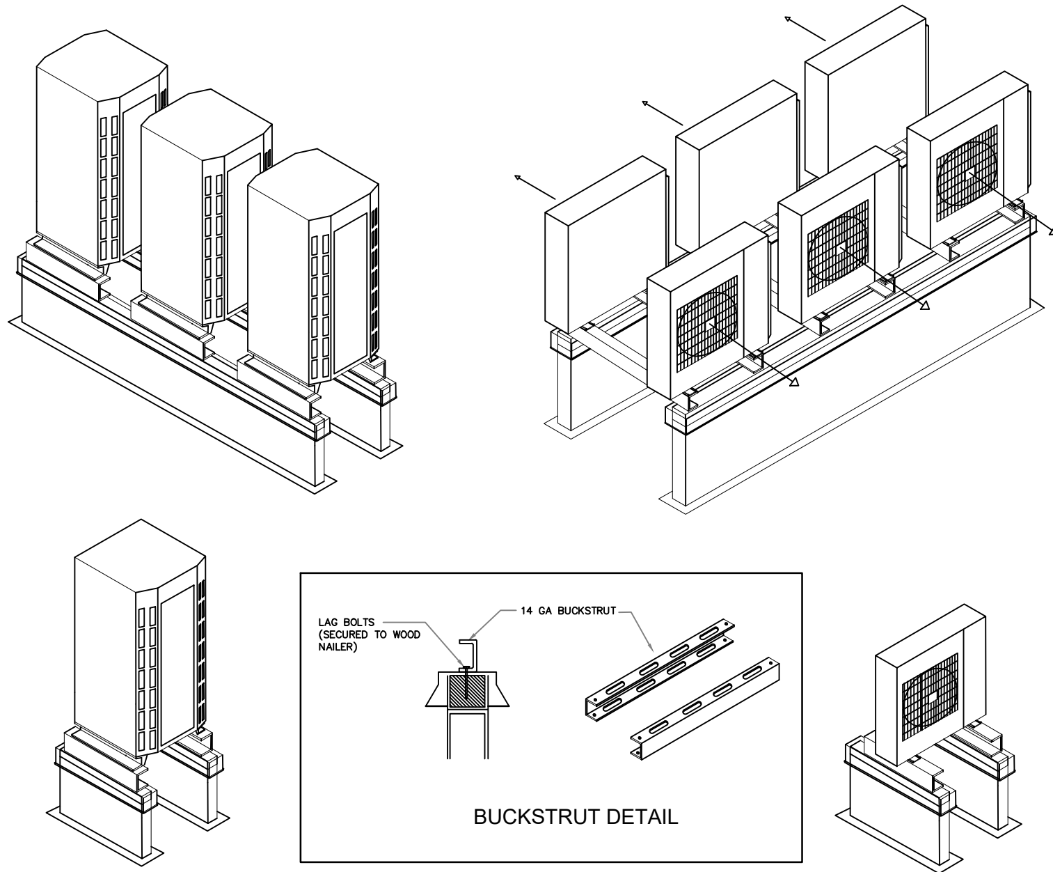
VRF CONDENSER SUPPORT BASE
